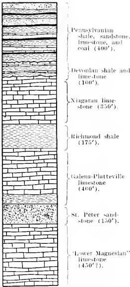
FIG. 15. Section showing rock formations that are penetrated by the deepest wells of the northern part of the area.
